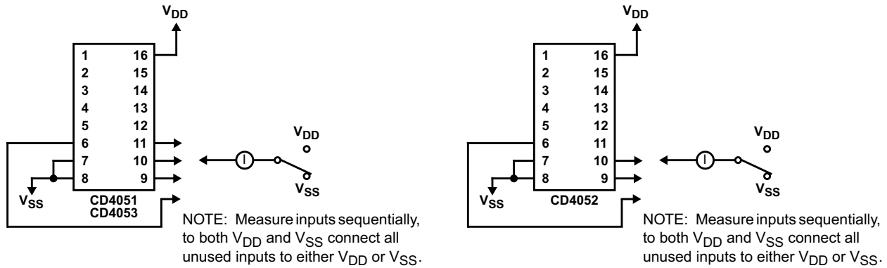
Figure 6-12. Input Current
